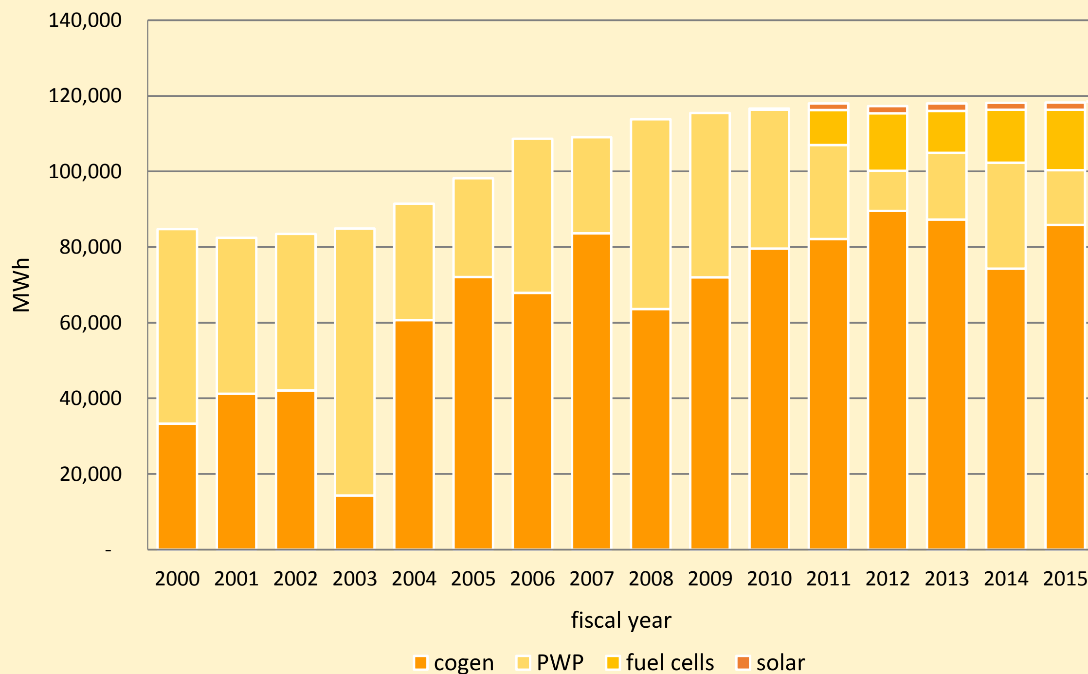
historic electricity consumption by source
